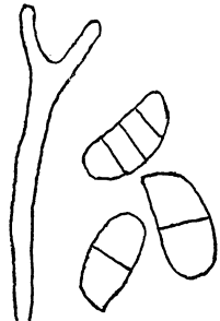
Fig. 5. D. pedunculata . Basidium and spores of type × 665.
